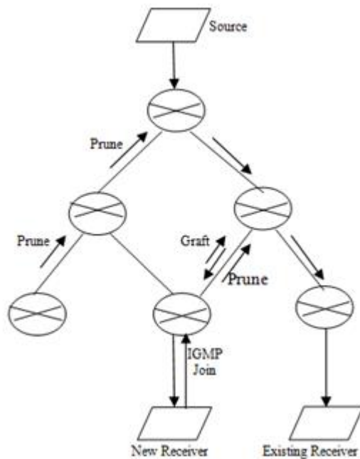
Figure 3 Message flowing in DVMRP
